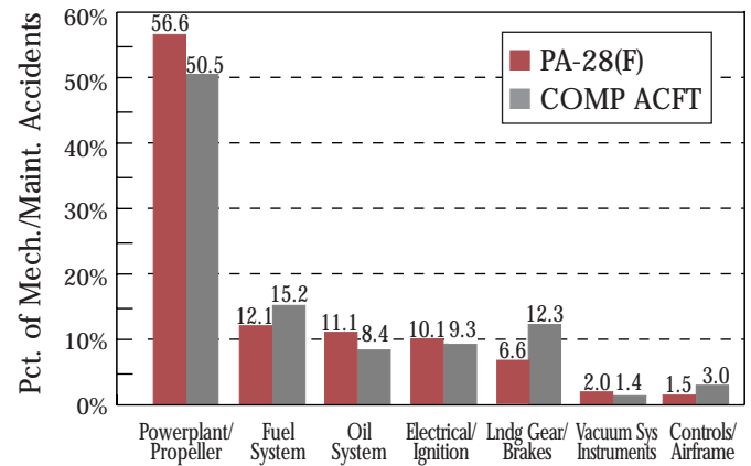
Figure 8. System Involvement PA-28(F)
